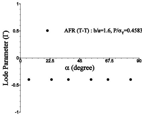
Fig. 17. Variation of Lode parameter versus variation of angle for perfect-plastic behavior of material and Tresca criterion.
