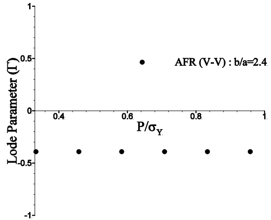
Fig. 12. Variation of Lode parameter in outer surface of the vessel with increasing the internal pressure for perfect-plastic behavior of material and von Mises criterion.
