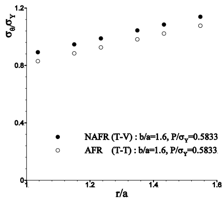
Fig. 11. A comparison between (V - T) and (T - V) for circumferential stress distributions, linear hardening.
