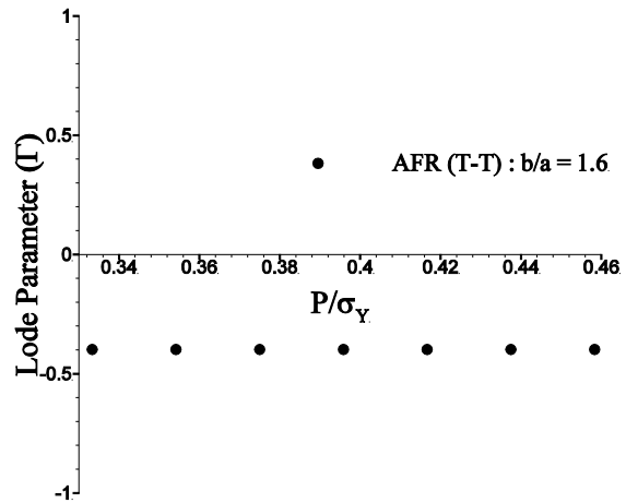
Fig. 15. Variation of Lode parameter in outer surface of the vessel because of increasing the internal pressure for perfect-plastic behavior of material and Tresca criterion.
