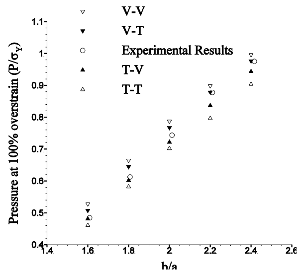
Fig. 3. A Comparing the experimental results and (V-V), (V-T), (T-V), (T-T).
