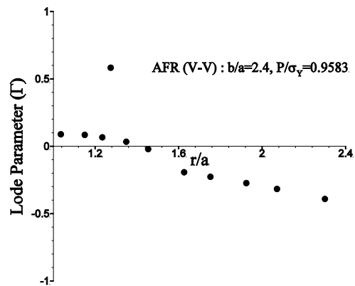
Fig. 13. Variation of Lode parameter with radius for perfect-plastic behavior of material and von Mises criterion.
