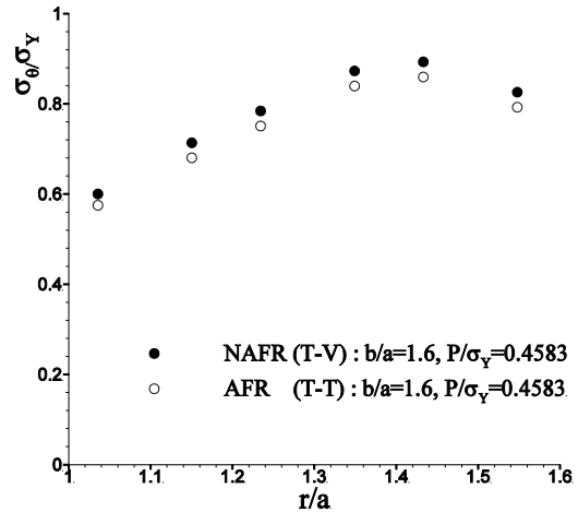
Fig. 9. Comparing (V - T) and (T - V) for circumferential stress distributions, perfect plastic.
