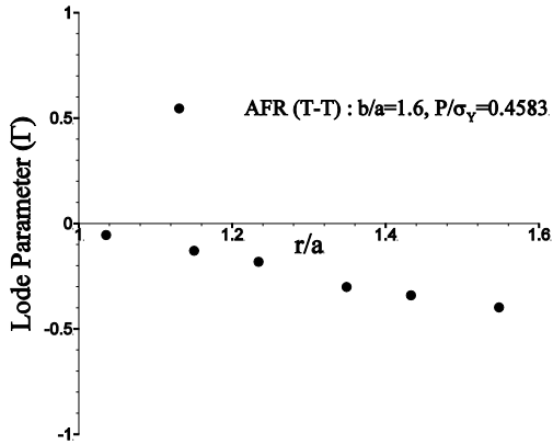
Fig. 16. Variation of Lode parameter versus the variation of radius for perfect-plastic behavior of material and Tresca criterion.
