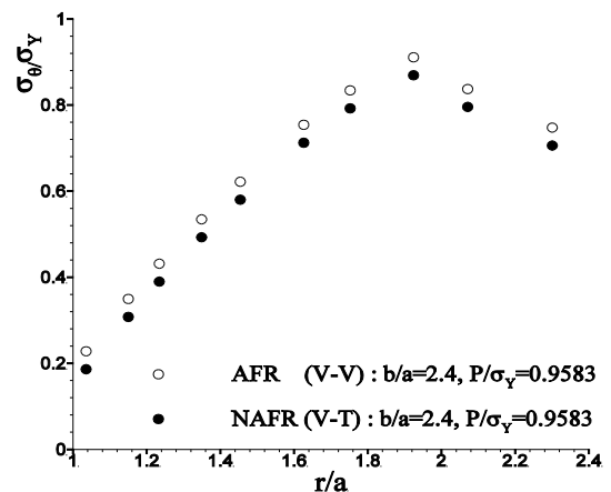
Fig. 5. Comparing (V - T) and (T - V) for circumferential stress distributions, perfect plastic.
