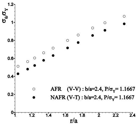
Fig. 7. Comparing (V - T) and (T - V) for circumferential stress distributions, linear hardening.
