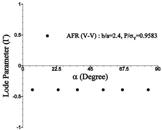
Fig. 14. Variation of Lode parameter versus variation of angle for perfect-plastic behavior of material and von Mises criterion.
