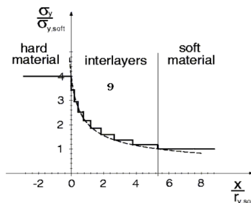
Fig. 2. Strength distribution in layers [5].
