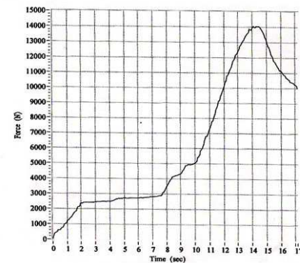
Fig. 7. Compression test for pure sulfur concrete (force versus time).
