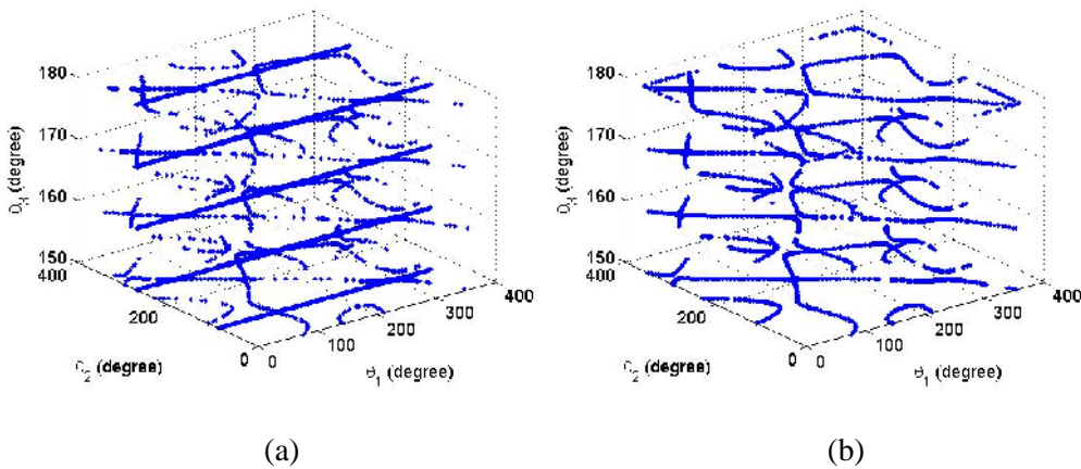
Fig. 3. Singularity contours while operation range of platform is 0^\circ \leq \theta_1, \theta_2 \leq 360^\circ, 150^\circ \leq \theta_3 \leq 180^\circ , (a) based on Euler angles and (b) based on Euler parameters.
