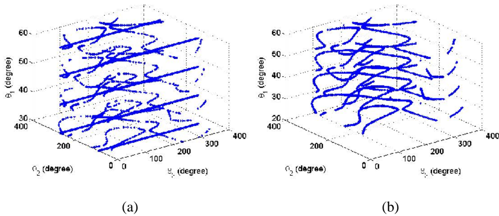
Fig. 2. Singularity contours while operation range of platform is 30^\circ \leq \theta_1 \leq 60^\circ, 0^\circ \leq \theta_2, \theta_3 \leq 360^\circ , (a) based on Euler angles and (b) based on Euler parameters.
