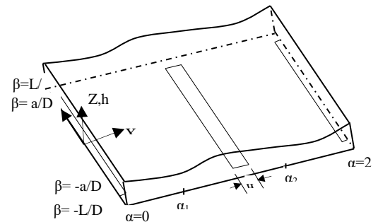
Fig. 3. Three dimensional view of fluid film between journal and bearing.
