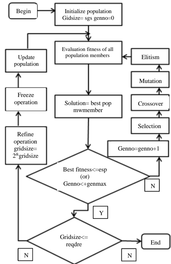
Fig. 8. The binary coded genetic algorithm reconstruction procedure (sgs: starting grid size).
