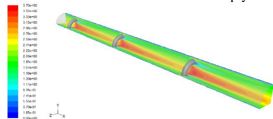
Fig. 13. Distribution of velocity in symmetry plates.
