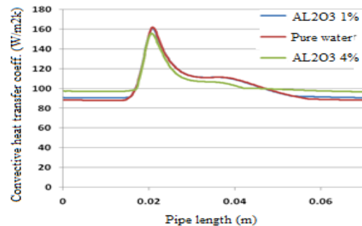
Fig. 9. Distribution of the heat transfer coefficient of the wall according to the pipe length for water/AL 2 O 3 nanofluid.
