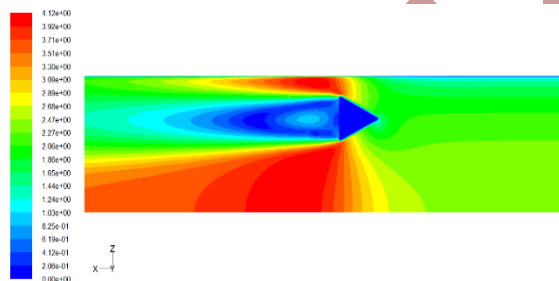
Fig. 6. Distribution of the velocity around the obstacle with a triangular cross section on the symmetry plate.
