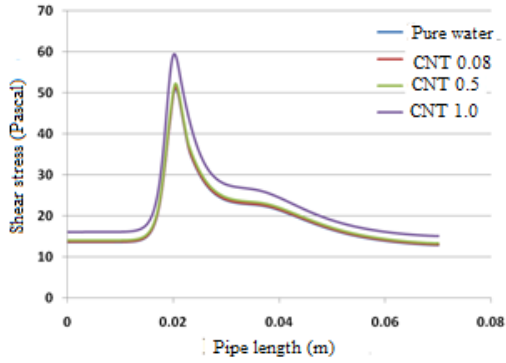
Fig. 10. Shear stress distribution of tube wall for pure water and water/CNT nanofluid with different percentages.
