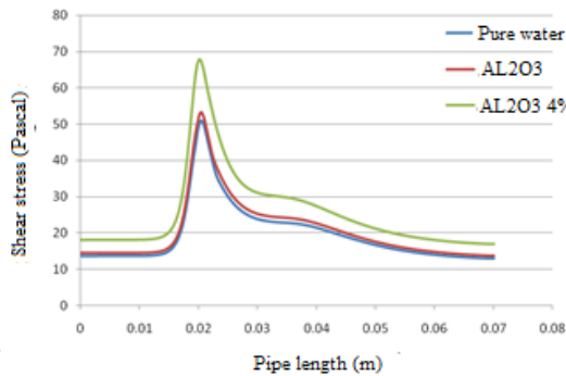
Fig. 11. Shear stress distribution of tube wall for pure water and water/AL 2 O 3 nanofluid with different percentages.
