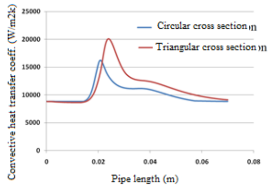
Fig. 7. Comparison of the distribution of the convection heat transfer coefficient in terms of pipe length of the circular and triangular barrier.
