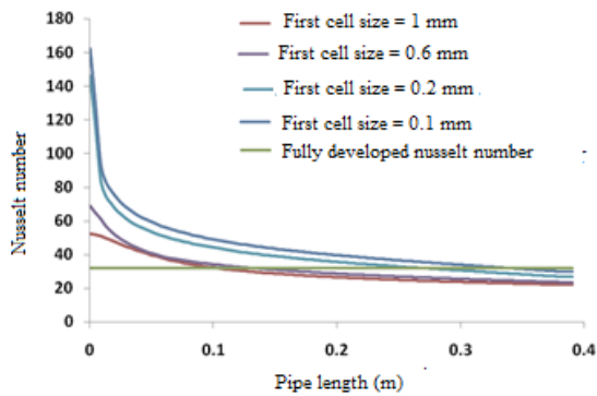
Fig. 3. Distribution of nusselt number of tube wall according to pipe length in different networks.
