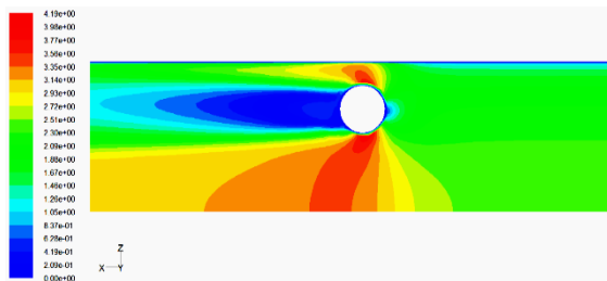
Fig. 5. Distribution of the velocity around the obstacle with a circular cross section on the symmetry plate.
