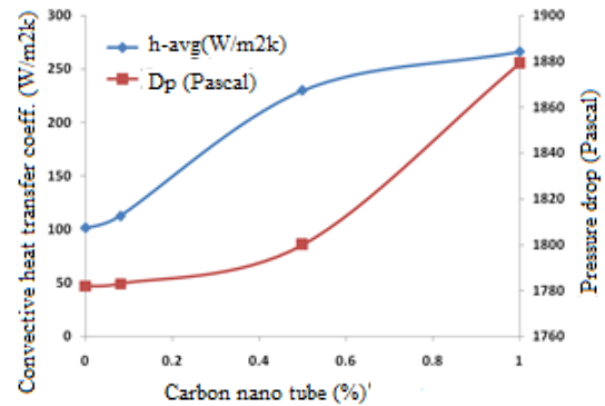
Fig. 12. The average heat transfer coefficient of the wall and the pressure drop in water/CNT nanofluid with different percentages.
