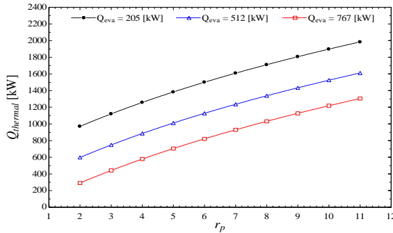
Fig. 13. Heating load as function of compressor pressure ratio and three different cooling capacity of absorption chiller.
