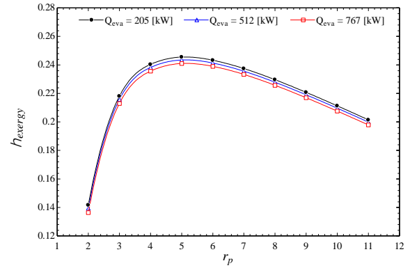
Fig. 16. Total exergy efficiency of the system as function of compressor pressure ratio and three different cooling capacity of absorption chiller
