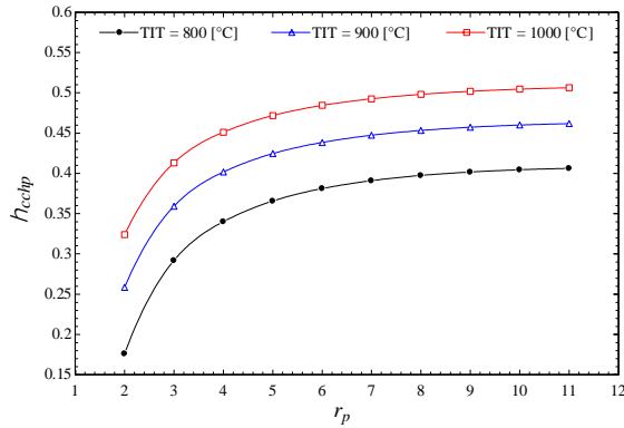
Fig. 8. Combined heating, cooling and power efficiency as function of compressor pressure ratio
