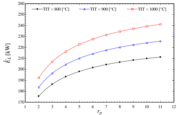
Fig. 12. Lost exergy rate of the system as function of compressor pressure ratio.
