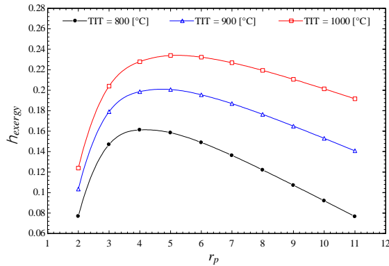
Fig. 9. Total exergy Efficiency of the System as function of compressor pressure ratio
