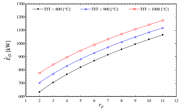
Fig. 11. Destroyed exergy rate of the system as function of compressor pressure ratio.
