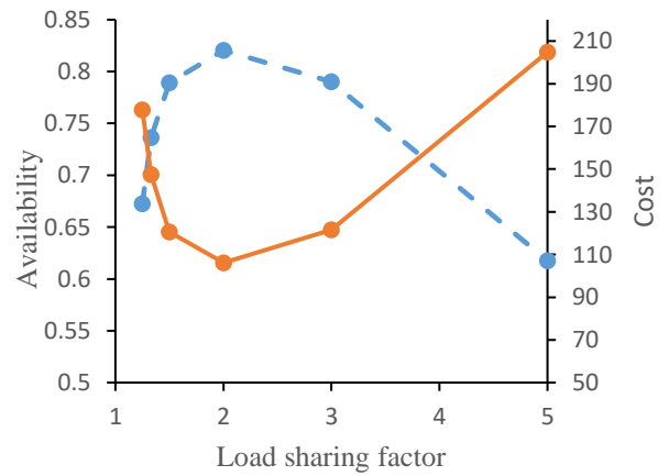
Fig. 17. Influence of load sharing factor on the cost and availability of an MSLSS with 80% output
