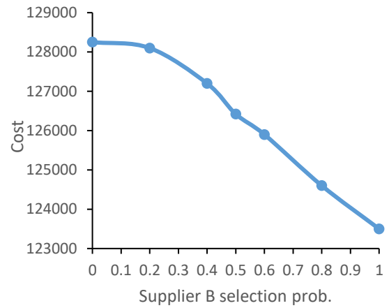
Fig. 5. Supplier selection influence on the system cost-case 2
