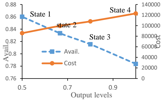
Fig. 12. The cost and availability of the MSLSS at different level outputs
