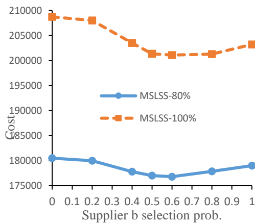
Fig. 16. Supplier selection influence on an MSLSS cost (configuration 2)
