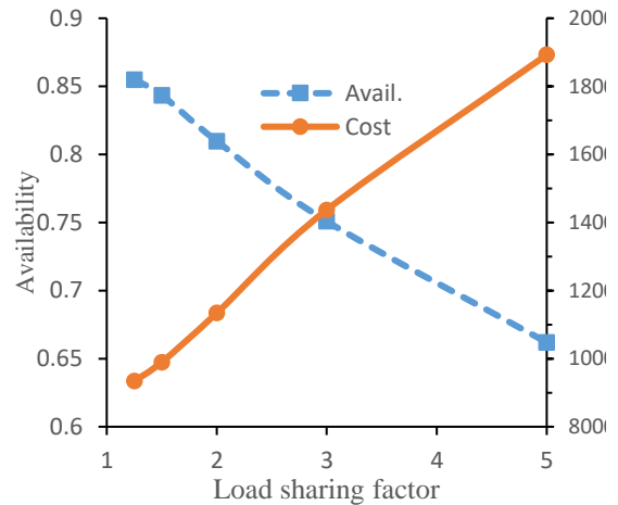
Fig. 11. Load-sharing factor influence on the system cost and availability- case 3
