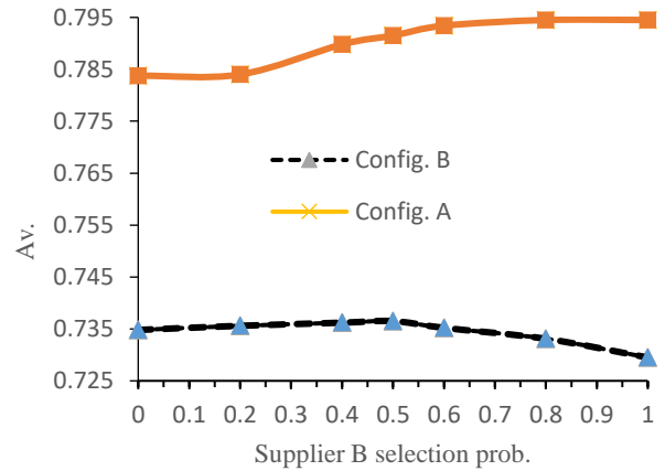
Fig. 8. System configuration and supplier influence on the availability
