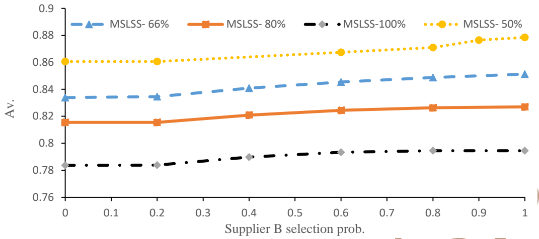
(a) Supplier selection influence on an MSLSS availability
