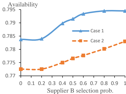
Fig. 7. Supplier selection influence on the system availability
