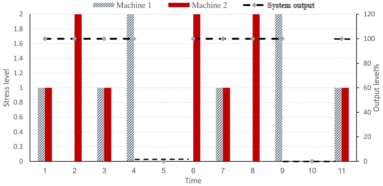
Fig. 1. Stress variation for a simple two-machines load-sharing system
