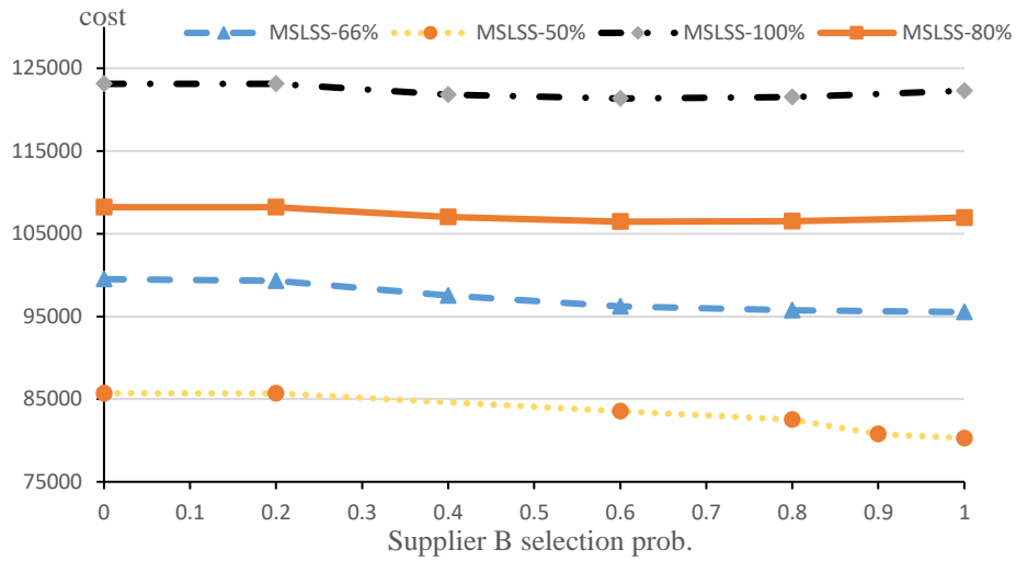
(b) Supplier selection influence on an MSLSS cost
