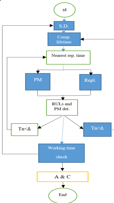
Fig. 2. An overall framework of the Monte Carlo simulation procedure
