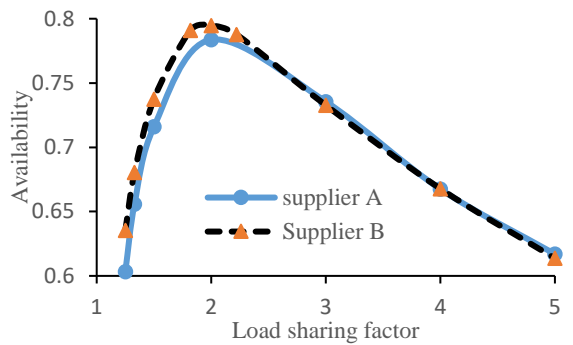
Fig. 10. Load-sharing influence on the system availability
