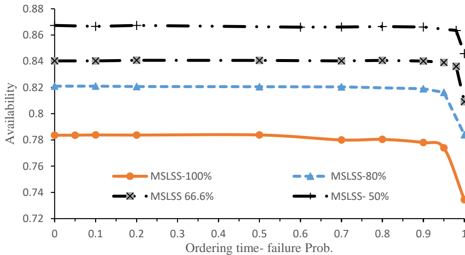
Fig. 13. The influence of ordering time on the availability for different levels of the MSLSS output
