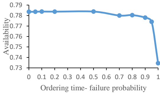
Fig. 4. Ordering time influence on the system availability
