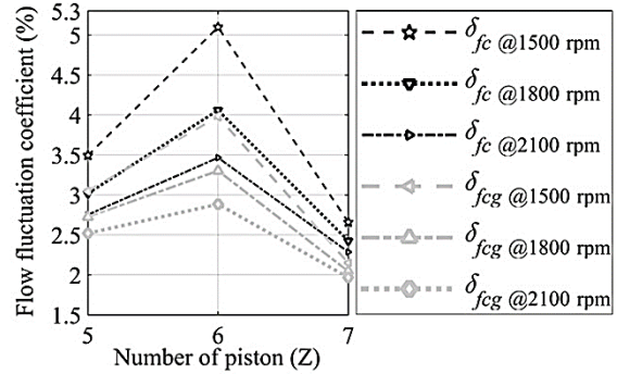
Fig. 7. Flow fluctuation coefficient with velocity variation.
