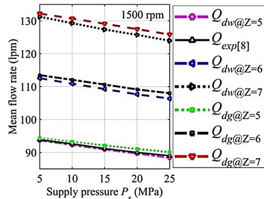
Fig. 6. Mean flow rate of the pump with supply pressure at the speed of 1500 rpm.
