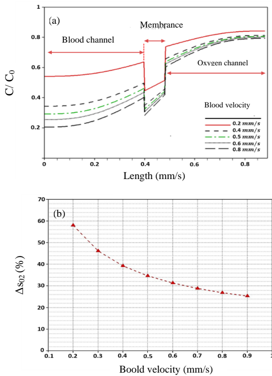
Fig. 4. (a) The oxygen concentration profile at the outlet of blood, membrane, and gas channels and (b) indicates the percentage of oxygen diffusivity into the bloodstream.
