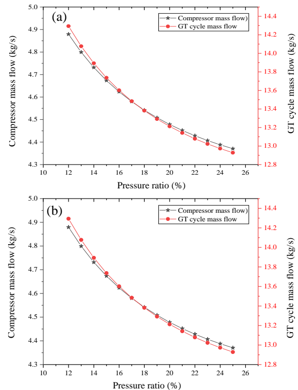
Fig. 5. GT PR relation to (a) turbine and (b) compressor mass flow.
