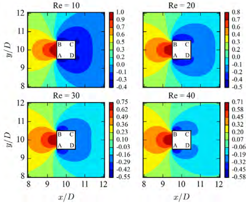
Fig. 5. Non-dimensional pressure ( \frac{P}{\rho U_{in}^2} ) around the square pile at different Reynolds numbers.
