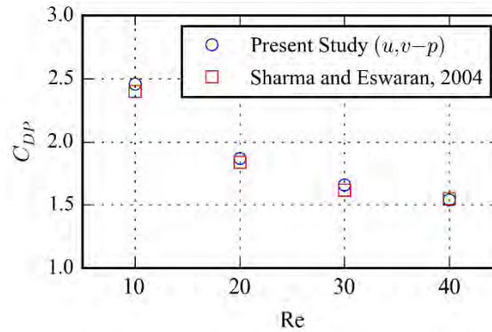
Fig. 6. Variation of the pressure drag coefficient with Reynolds number.
