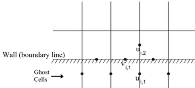
Fig. 3. An example of the applying boundary conditions in the staggered grid system.
