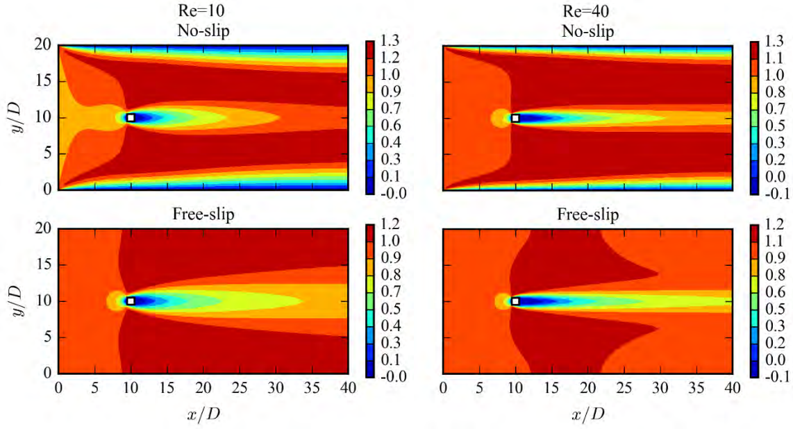
Fig. 10. The stream-wise velocity in the whole computational domain for different lateral boundary conditions.
