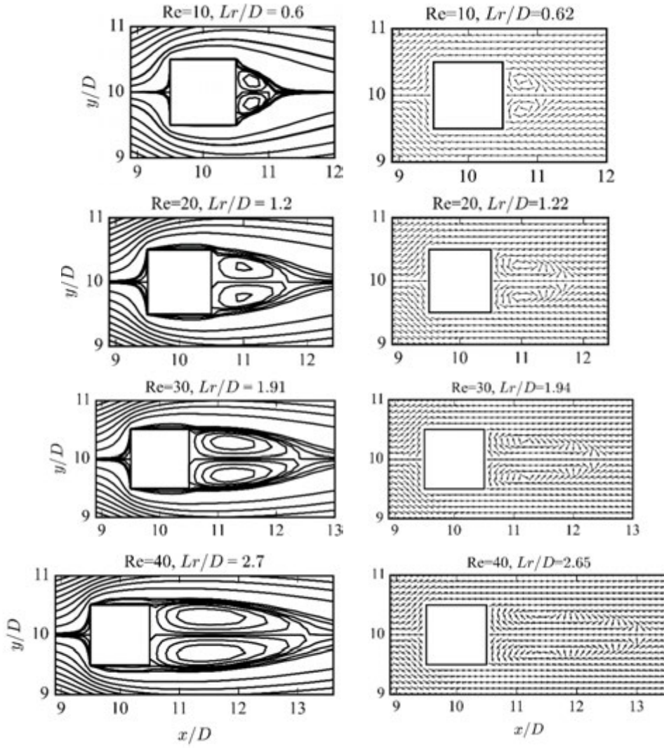
Fig. 7. Flow behavior around the square pile for various Reynolds numbers; Left : \omega-\psi formulation, Right : u, v-p formulation.
