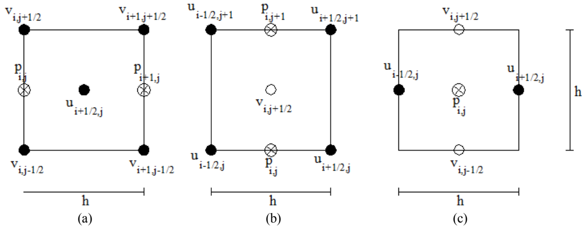
Fig. 2. Control volume for: (a) u -velocity, (b) v -velocity components, and (c) pressure.
