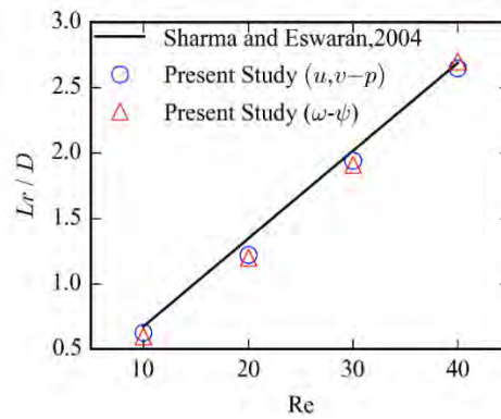
Fig. 8. Non-dimensional recirculation length for various Reynolds numbers.
