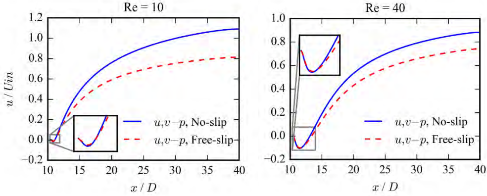
Fig. 11. The stream-wise velocity at the wake centerline for different lateral boundary conditions.
