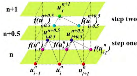
Fig. 3. Stencil of two-time steps LxW.
