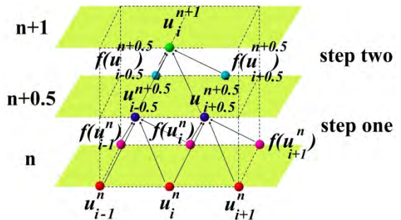
Fig. 2. The stencil of the two-time step LxF.
