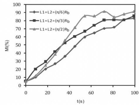
Fig. 8. Effect of the length of blades on mixing index ( \omega_{ave} = 15 rpm and \Delta\omega = 10 rpm for all cases).
